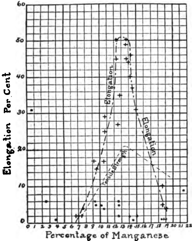
Fig. 84. Influence of the Proportion of Manganese on the Ductility of Manganese Steel.
